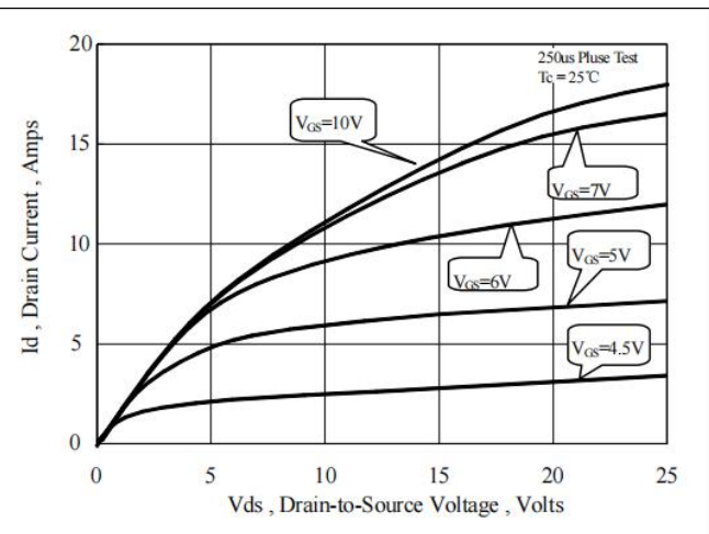
Figure 6. On-State Characteristics
