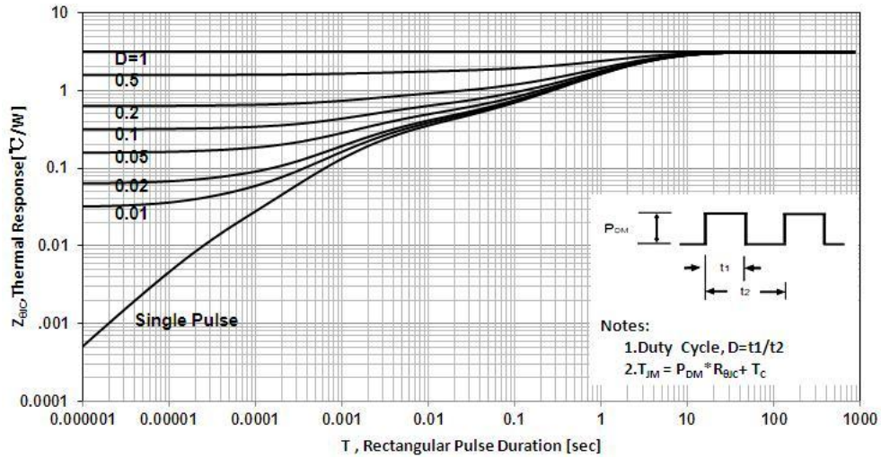
Figure 9. Maximum Effective Thermal Impedance , Junction to Case
